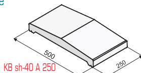
KB sh-40 A 250
